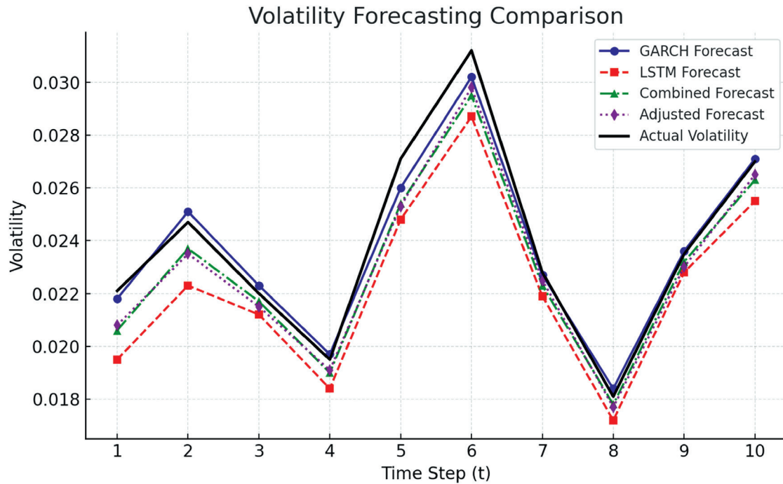
Figure 7. Comparison of volatility in forecasting
