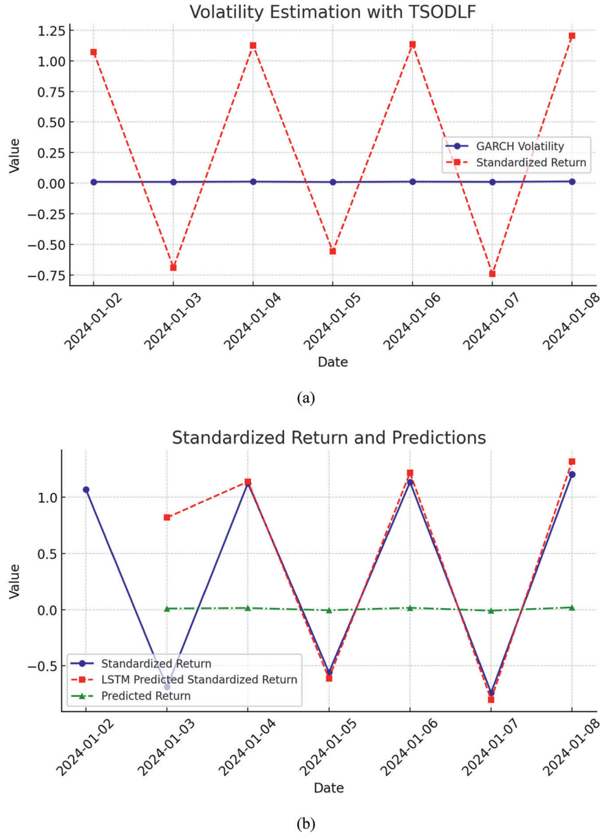
Figure 8. Time series estimation with TSODLF (a) volatility estimation (b) standardized return
