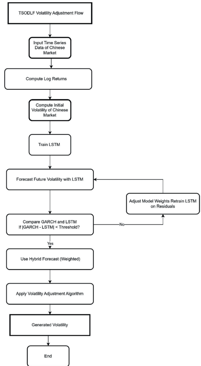
Figure 2. Flow chart of TSODLF
