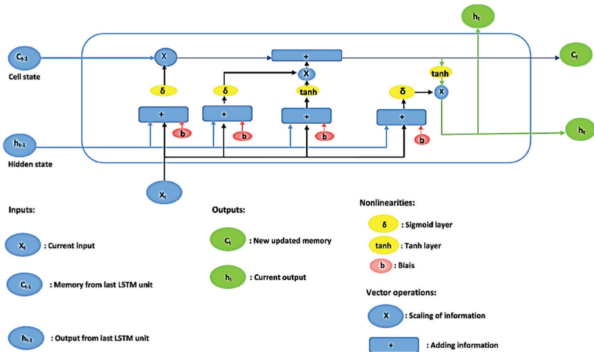
Figure 1. Architecture of the TSODLF
