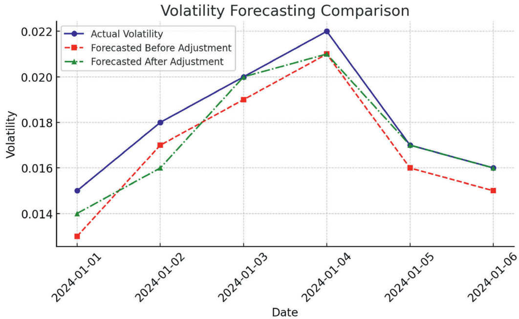
Figure 6. Volatility forecasting
