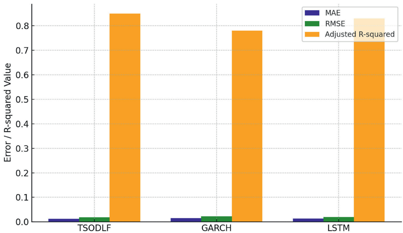
Figure 4. Error estimation with TSODLF
