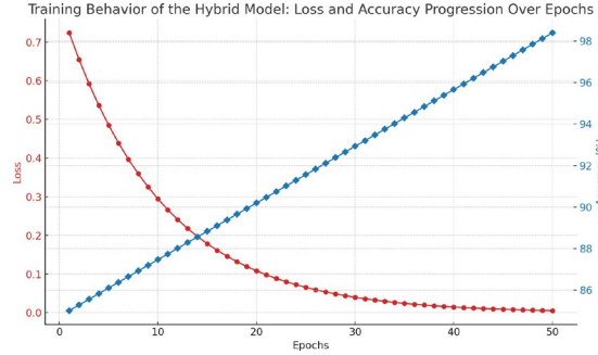
Fig. 2. Training behavior of the hybrid model: Loss and accuracy progression over epochs
