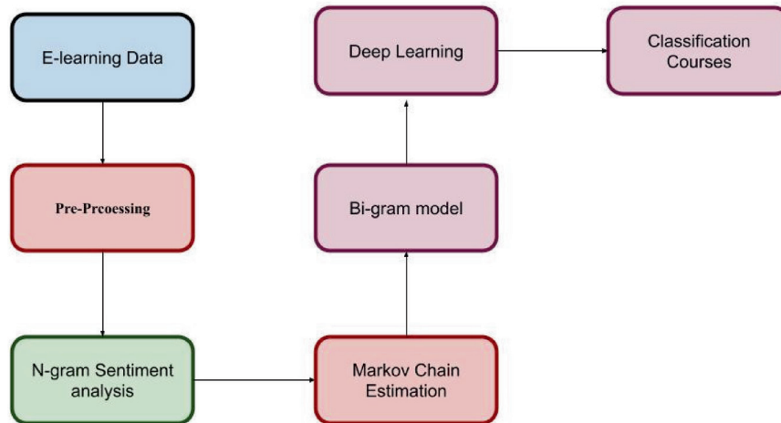
Figure 3. Flow chart of n-gram-LMS-MC-DL
