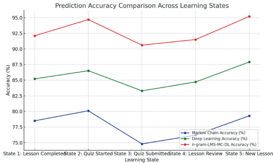
Figure 6. Prediction with n-gram-LMS-MC-DL
