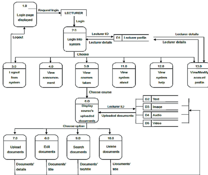
Figure 1. Learning management system with deep learning
