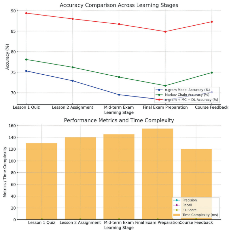
Figure 5. Course estimation with n-gram-LMS-MC-DL
