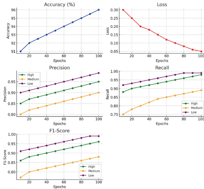
Figure 7. Classification with LMS with deep learning
